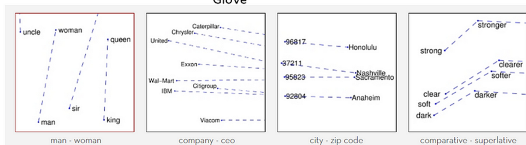
GloVe
