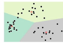
K-means clustering
