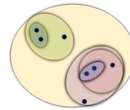
Hierarchical clustering
